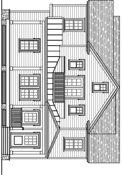
REAR ELEVATION
