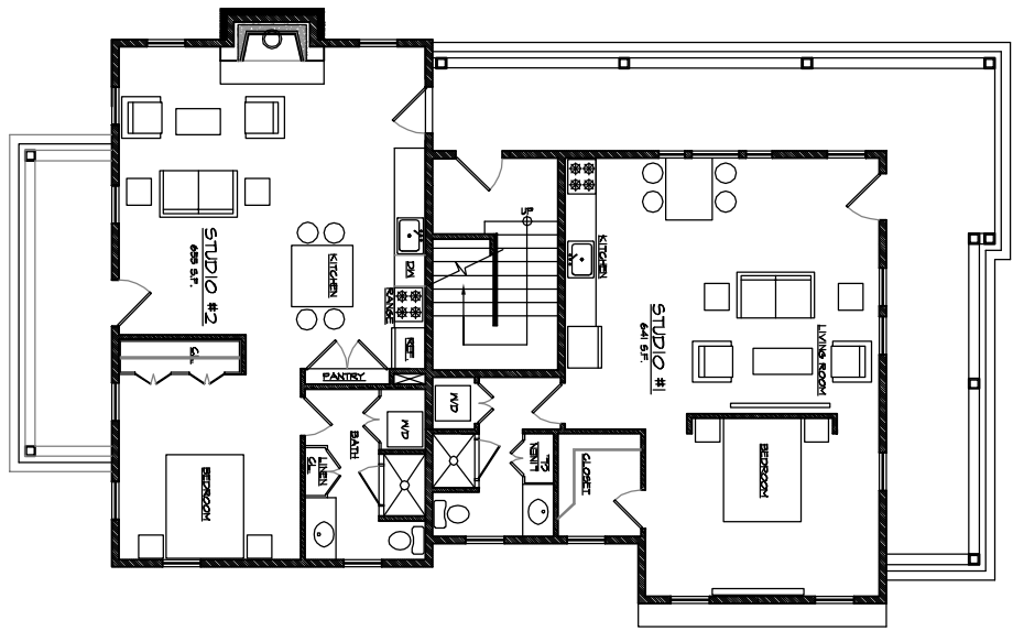
1st FLOOR 1/4"=1'-0"
