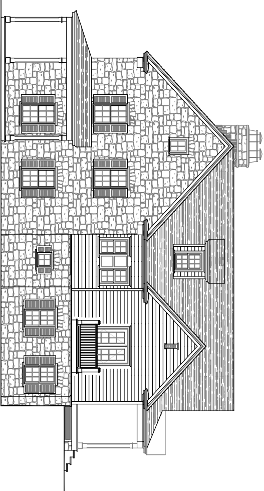
UNIT 'A' 4 BAY - RIGHT SIDE ELEVATION SCALE: 1/4"=1'-0"
