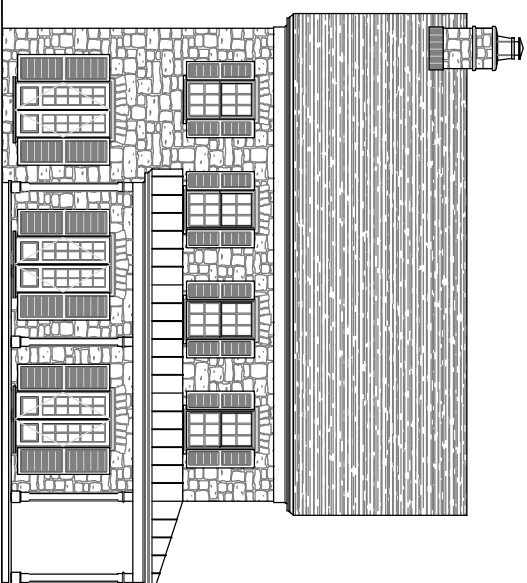
UNIT 'A' 4 BAY - FRONT ELEVATION SCALE: 1/4"=1'-0"
