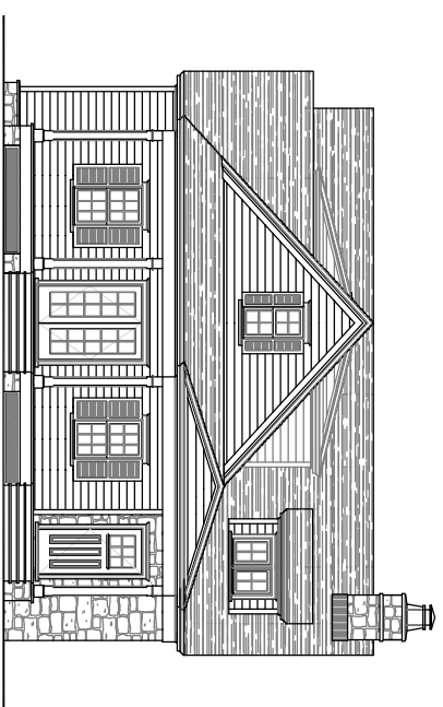
UNIT 'A' 4 BAY - REAR ELEVATION SCALE: 1/4"=1'-0"
